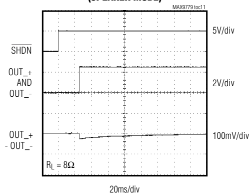
TURN-ON RESPONSE (SPEAKER MODE)
