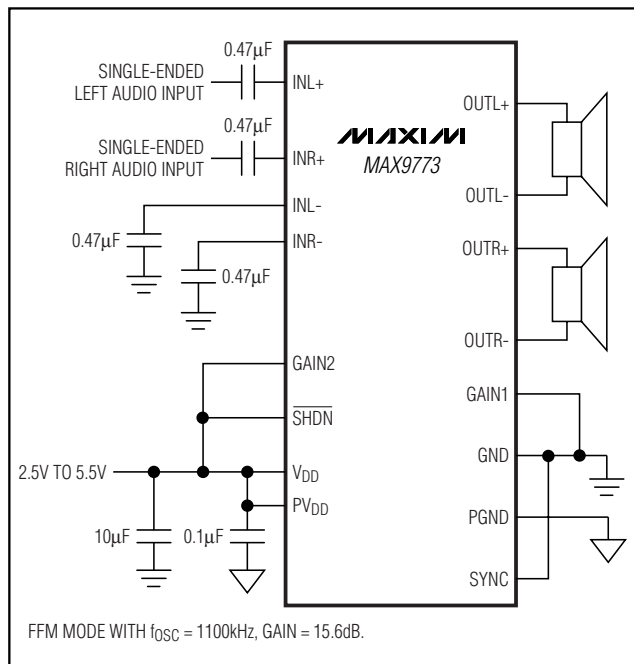
Figure 7. Single-Ended Input
