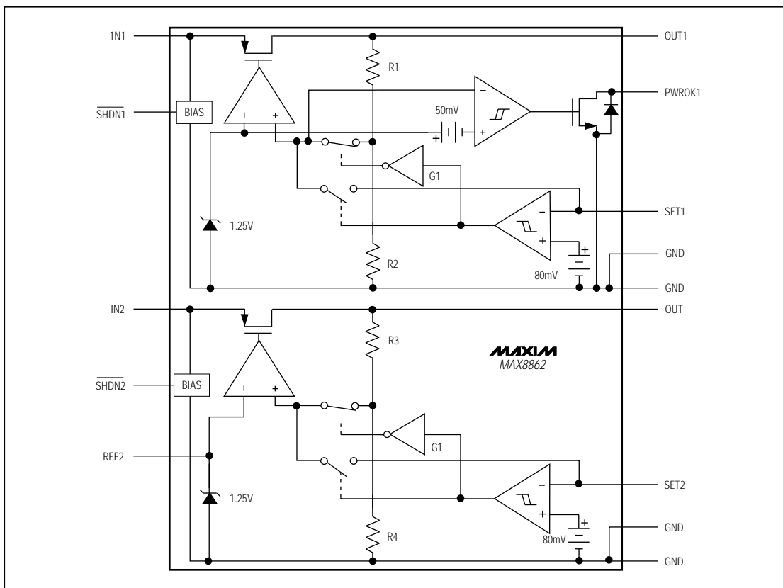
Figure 1. Functional Diagram
