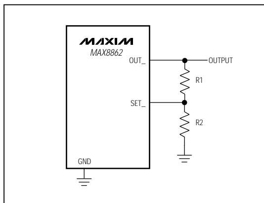
Figure 2. Adjustable Output Voltage
