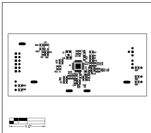
Figure 7. MAX8760 EV Kit Component Placement Guide—Solder Side
