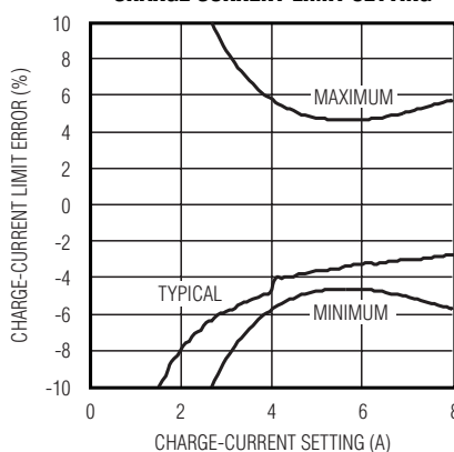
CHARGE-CURRENT ERROR vs. CHARGE CURRENT-LIMIT SETTING
