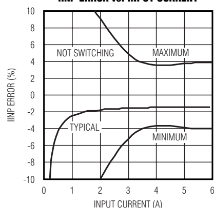
IINP ERROR vs. INPUT CURRENT
