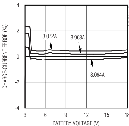
CHARGE-CURRENT ERROR vs. BATTERY VOLTAGE
