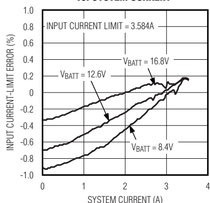
INPUT CURRENT-LIMIT ERROR vs. SYSTEM CURRENT
