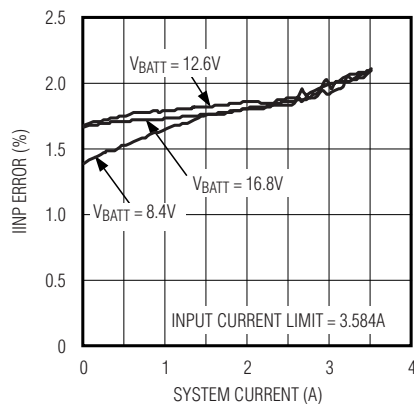
IINP ERROR vs. SYSTEM CURRENT
