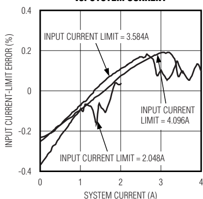
INPUT CURRENT-LIMIT ERROR vs. SYSTEM CURRENT
