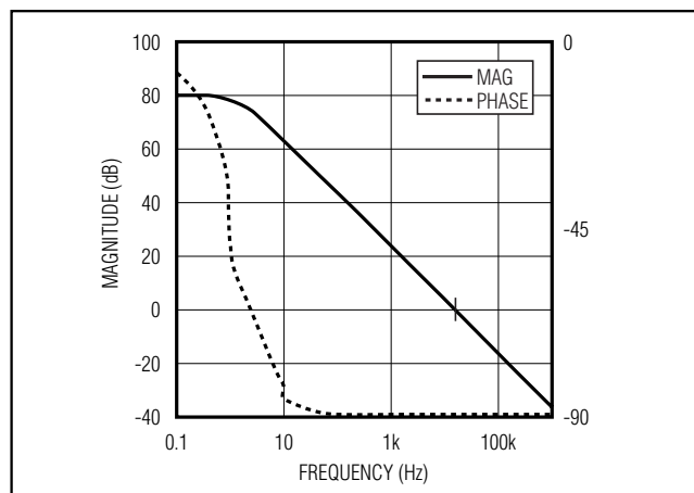
Figure 10. CCI Loop Response
