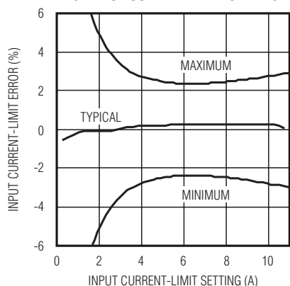
INPUT CURRENT-LIMIT ERROR vs. INPUT CURRENT-LIMIT SETTING
