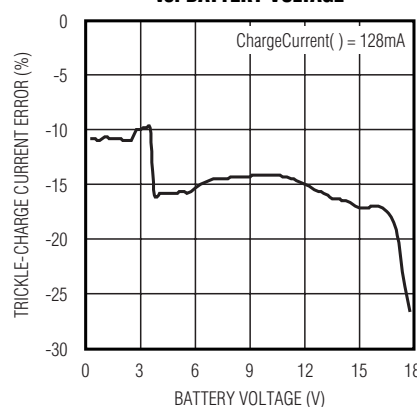
TRICKLE-CHARGE CURRENT ERROR vs. BATTERY VOLTAGE
