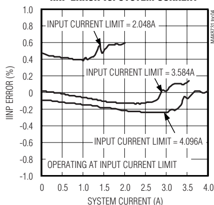
IINP ERROR vs. SYSTEM CURRENT
