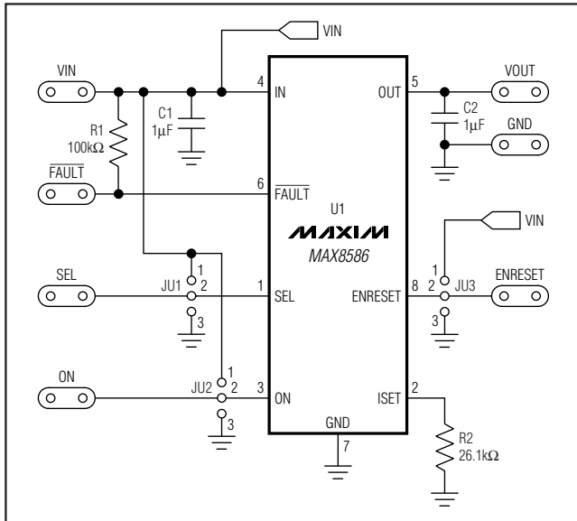
Figure 1. MAX8586 EV Kit Schematic
