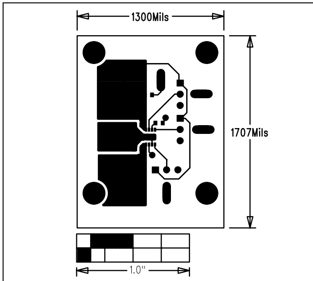
Figure 3. MAX8586 EV Kit PC Board Layout—Component Side
