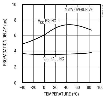
MAX793/MAX794 LOWLINE COMPARATOR PROPAGATION DELAY vs. TEMPERATURE
