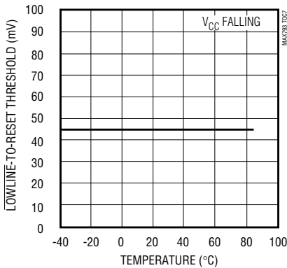
MAX793 LOWLINE-TO-RESET THRESHOLD vs. TEMPERATURE
