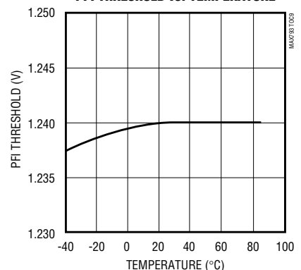
MAX793/MAX794 PFI THRESHOLD vs. TEMPERATURE
