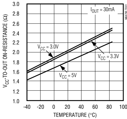
V_{CC} -TO-OUT ON-RESISTANCE vs. TEMPERATURE
