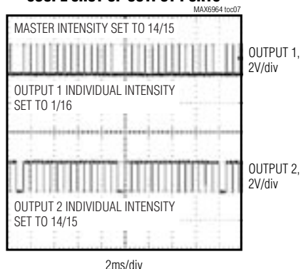
SCOPE SHOT OF OUTPUT PORTS
