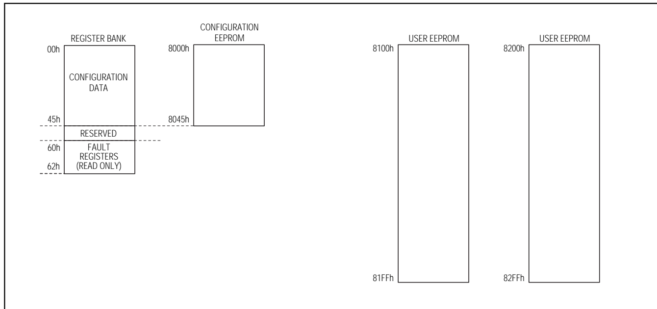
Figure 8. Memory Map
