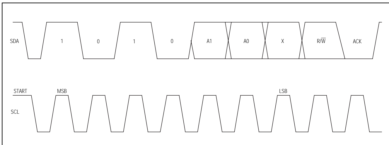
Figure 6. Slave Address
