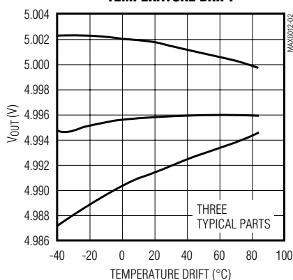
MAX6050 OUTPUT VOLTAGE TEMPERATURE DRIFT
