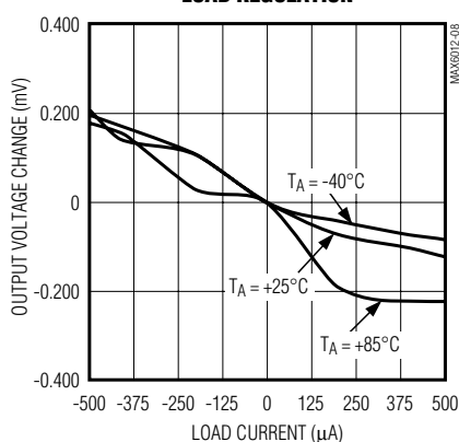
MAX6050 LOAD REGULATION
