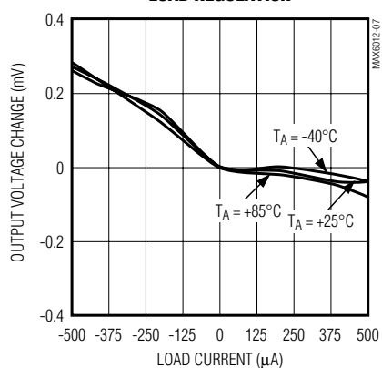
MAX6012 LOAD REGULATION
