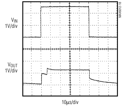
MAX6012 TURN-ON TRANSIENT
