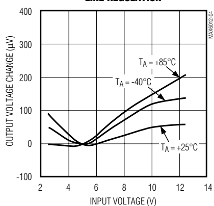
MAX6012 LINE REGULATION
