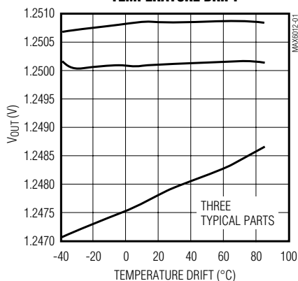
MAX6012 OUTPUT VOLTAGE TEMPERATURE DRIFT
