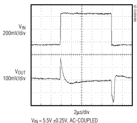
MAX6050 LINE-TRANSIENT RESPONSE
