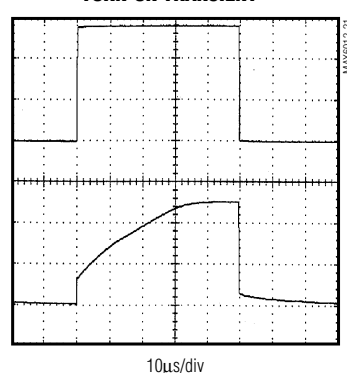
MAX6050 TURN-ON TRANSIENT
