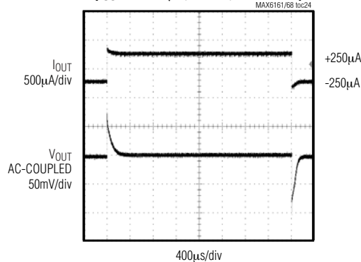
MAX6165 LOAD TRANSIENT ( I_{OUT} = \pm 250\mu A , C_L = 0 , V_{IN} = 5.5V )
