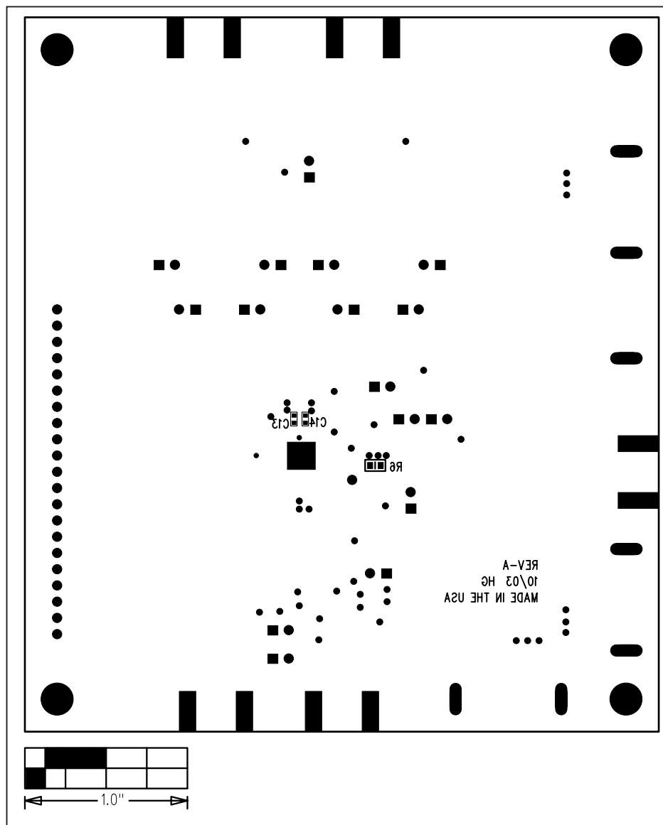
Figure 9. MAX5858A EV Kit Component Placement Guide—Solder Side
