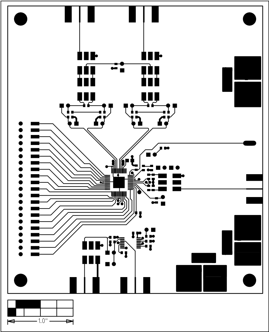
Figure 5. MAX5858A EV Kit PC Board Layout—Component Side
