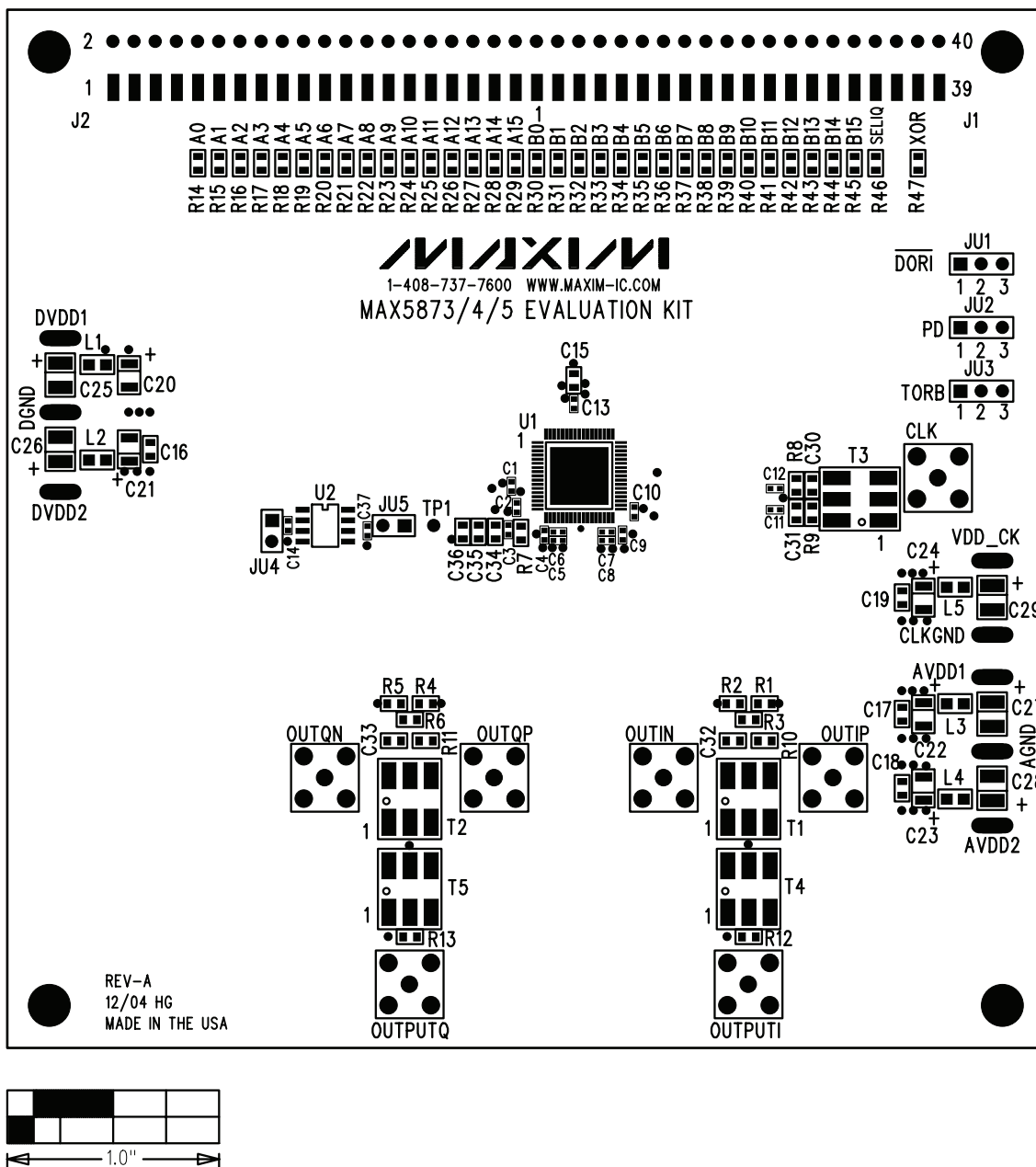
Figure 3. MAX5875 EV Kit Component Placement Guide—Component Side
