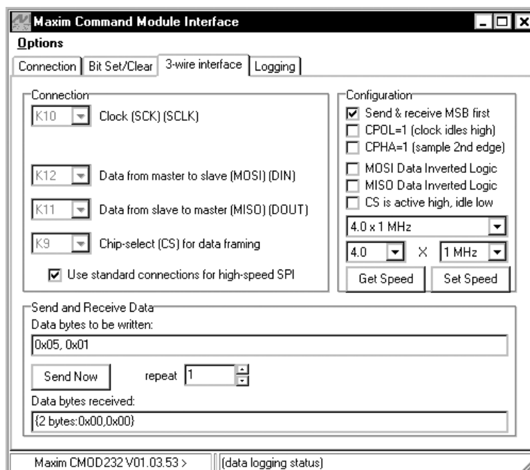
Figure 4. The above example shows a simple SPI transfer operation using the included 3-Wire Interface Diagnostics. In this example, the software is writing data (0x01h) to register address 0x05h. This sets the IDAC coarse gain to 1.
