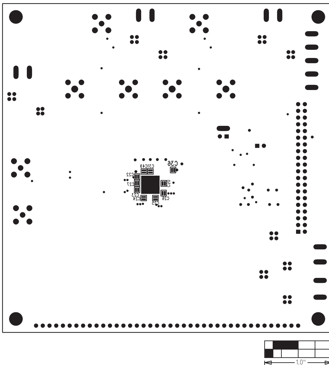
Figure 11. MAX5893/MAX5894/MAX5895 EV Kit Component Placement Guide—Solder Side
