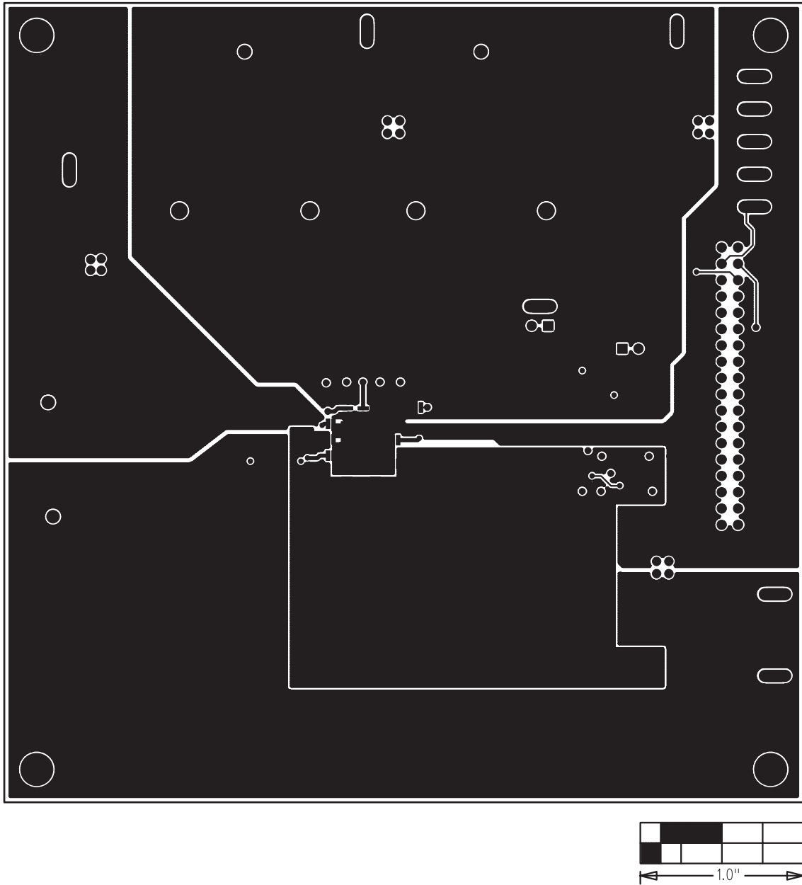
Figure 10. MAX5893/MAX5894/MAX5895 EV Kit PC Board Layout—Solder Side
