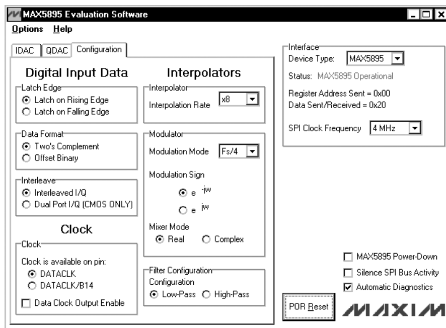
Figure 3. MAX5895 EV Kit Software Main Window (Configuration Tab)
