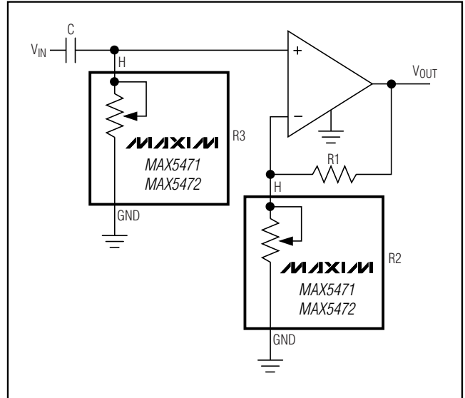
Figure 6. Programmable Filter
