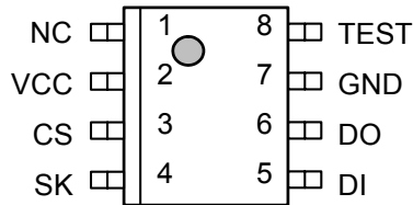
8-Pin SOP(JEDEC) (翻转版) Top view
