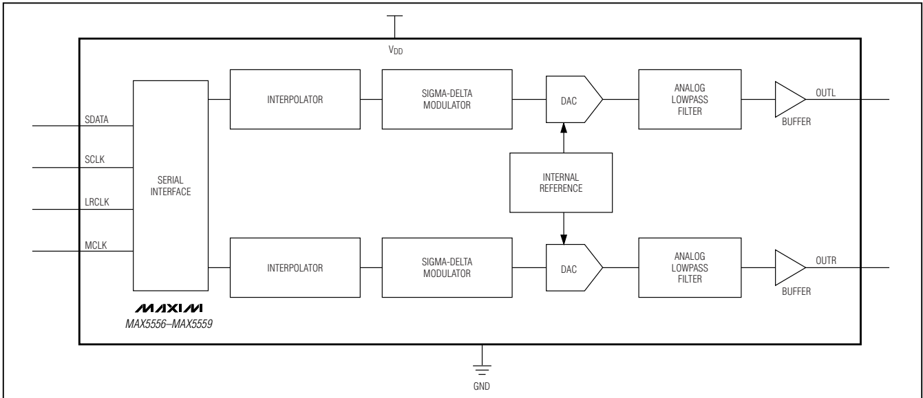
Figure 2. Functional Diagram
