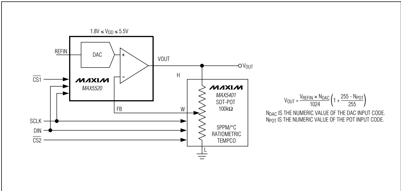
Figure 10. Software-Configurable Output Gain
