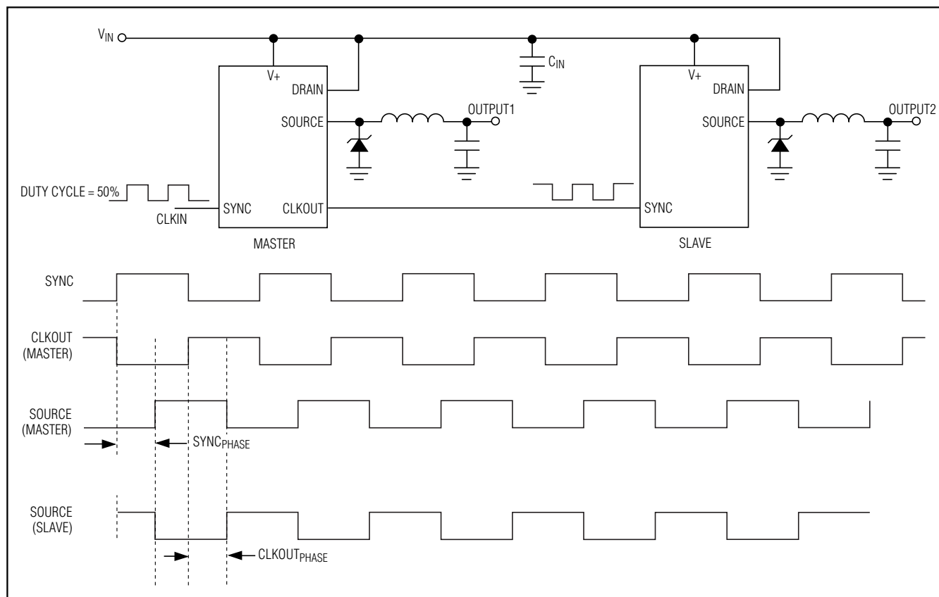
Figure 7. Synchronized Converters
