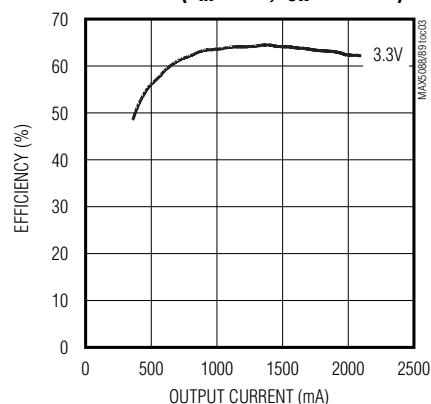
MAX5088 BUCK EFFICIENCY vs. OUTPUT CURRENT ( V_{IN} = 16V , f_{SW} = 2.2MHz )
