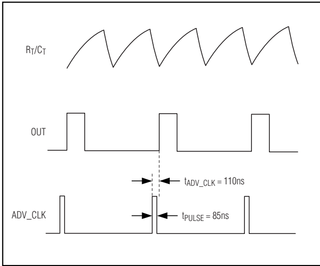
Figure 4. ADV_CLK
