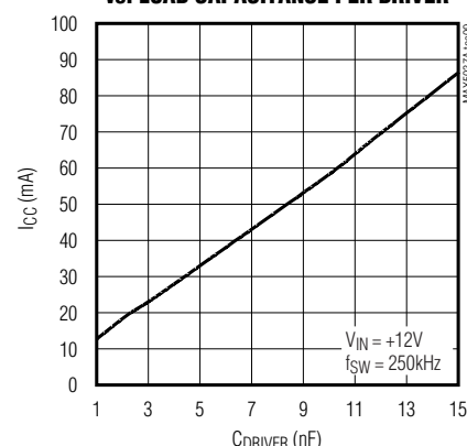
SUPPLY CURRENT vs. LOAD CAPACITANCE PER DRIVER
