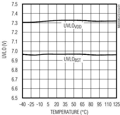
UNDervOLTAGE LOCKOUT ( V_{DD} AND V_{BST} RISING) vs. TEMPERATURE
