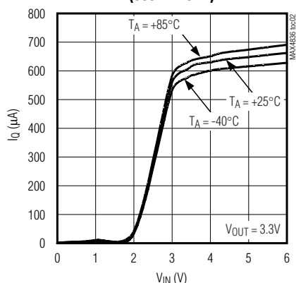
QUIESCENT CURRENT vs. INPUT VOLTAGE (500mA LOAD)
