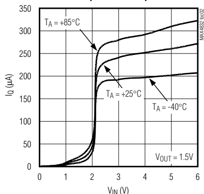
QUIESCENT CURRENT vs. INPUT VOLTAGE (100mA LOAD)
