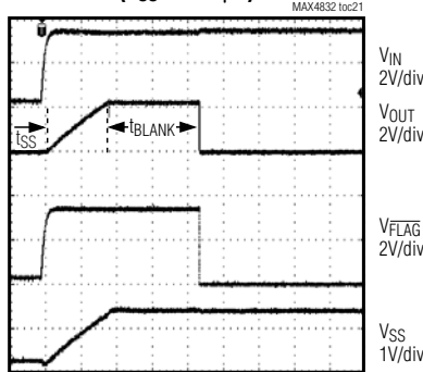
STARTUP IN AN OVERLOAD CONDITION (CSS = 0.01 \mu F)
