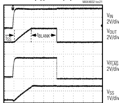
STARTUP IN AN OVERLOAD CONDITION (CSS = 0.01μF)
