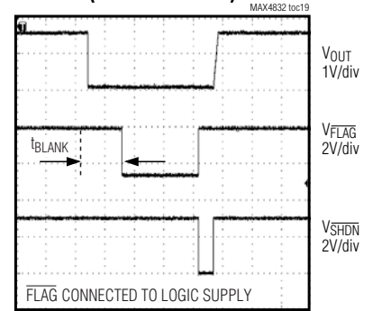
FLAG RESPONSE WHEN OUT IS SHORTED TO GND > BLANKING TIME (SHDN IS TOGGLED)
