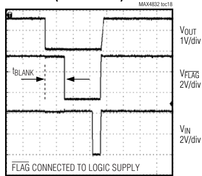
FLAG RESPONSE WHEN OUT IS SHORTED TO GND > BLANKING TIME (IN IS TOGGLED)
