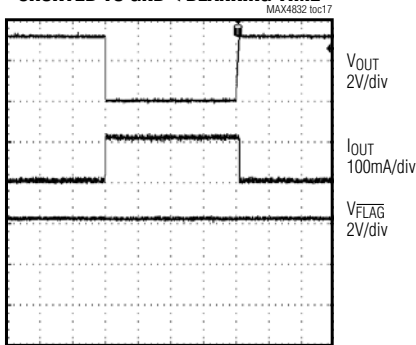
FLAG RESPONSE WHEN OUT IS SHORTED TO GND < BLANKING TIME
