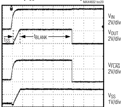
STARTUP IN AN OVERLOAD CONDITION (CSS NOT CONNECTED)
