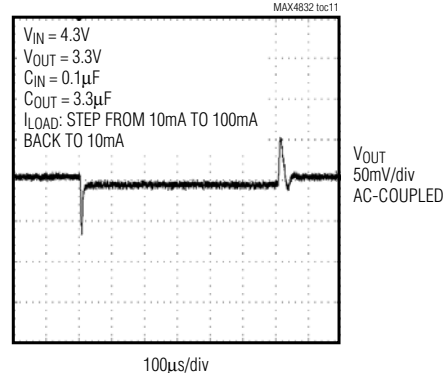
LOAD-TRANSIENT RESPONSE
