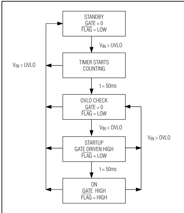
Figure 6. State Diagram
