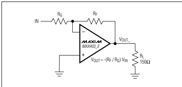
Figure 2. Inverting Gain Configuration
