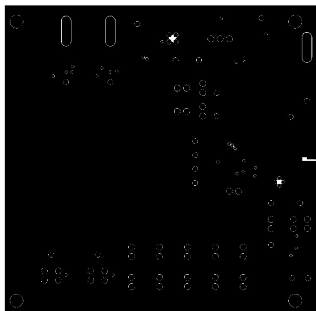
Figure 3. MAX3701 EV Kit PC Board Layout - Ground Plane
