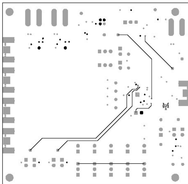
Figure 4. MAX3701 EV Kit PC Board Layout - Solder Side
