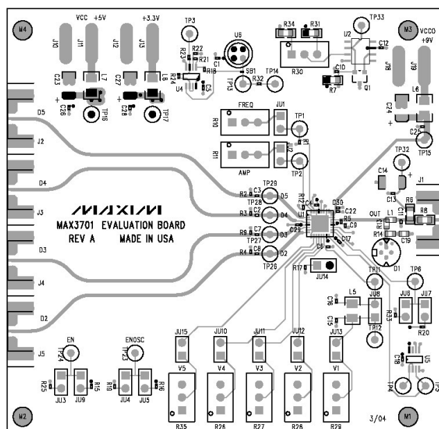
Figure 2. MAX3701 EV Kit Component Placement Guide - Component Side
