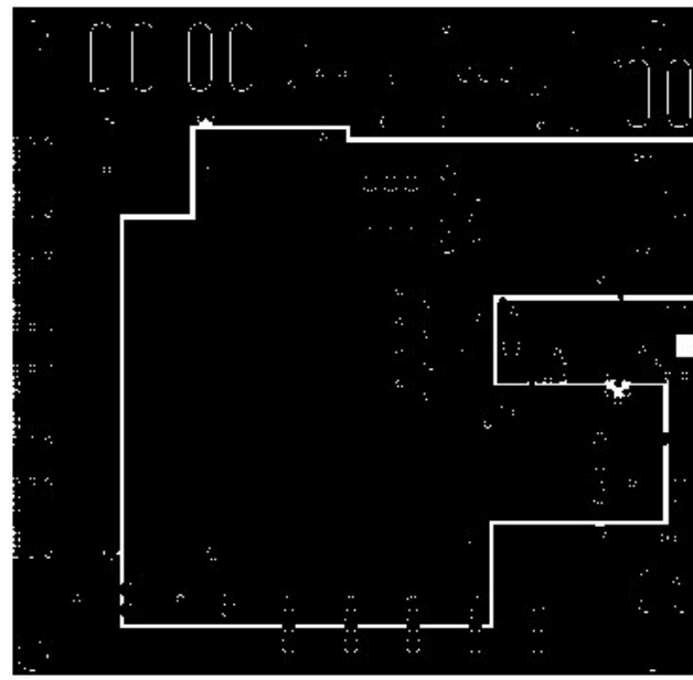
Figure 5. MAX3701 EV Kit PC Board Layout - Power Plane
