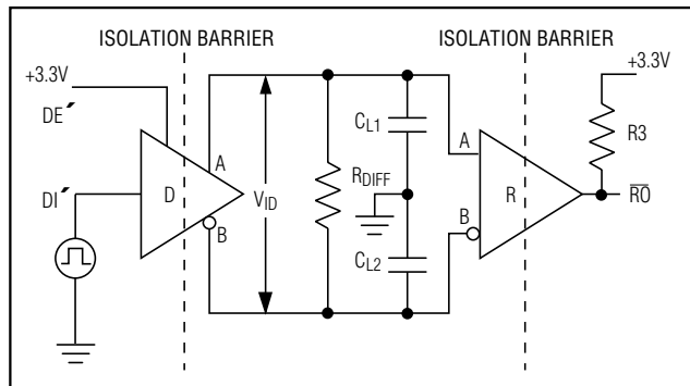
Figure 4. Driver/Receiver Timing Test Circuit
