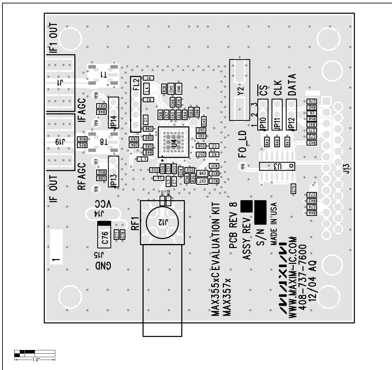
Figure 2. MAX355x/MAX357x EV PC Board Layout—Component Placement Guide
