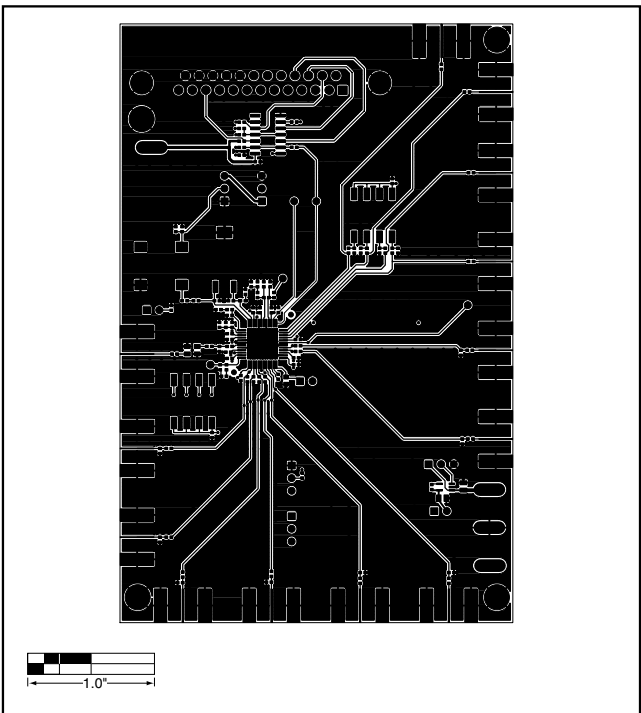
Figure 5. MAX2745 EV Kit PC Board Layout—Component Side
