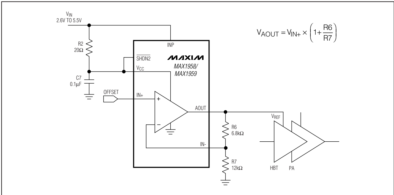
Figure 4. Op-Amp Configuration
