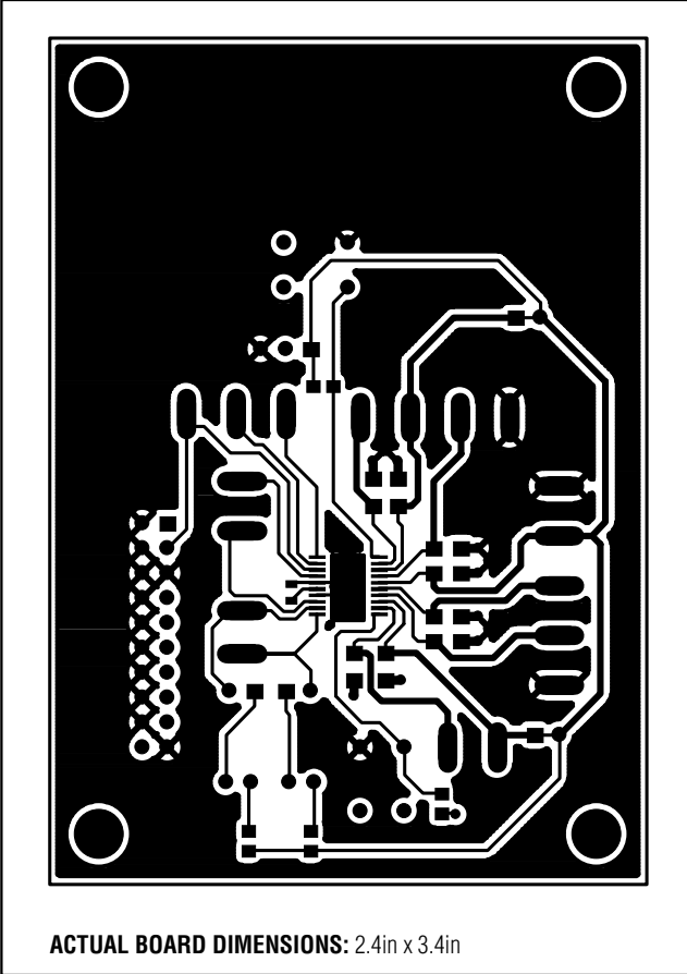
Figure 4. MAX1799 EV Kit PC Board Layout—Component Side
