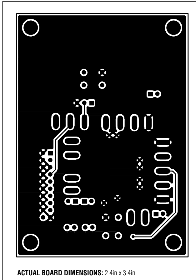
Figure 5. MAX1799 EV Kit PC Board Layout—Solder Side
