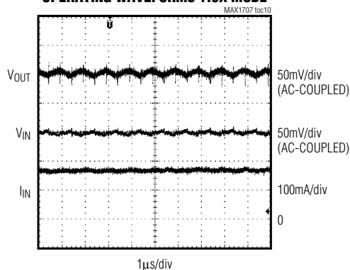
OPERATING WAVEFORMS 1.5X MODE
