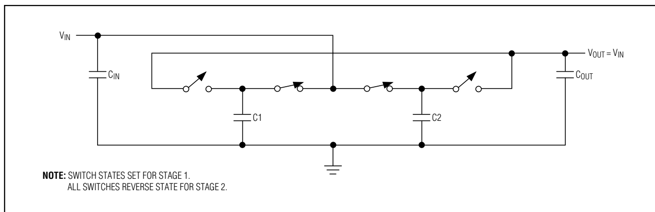
Figure 1. 1:1 Capacitor Configuration
