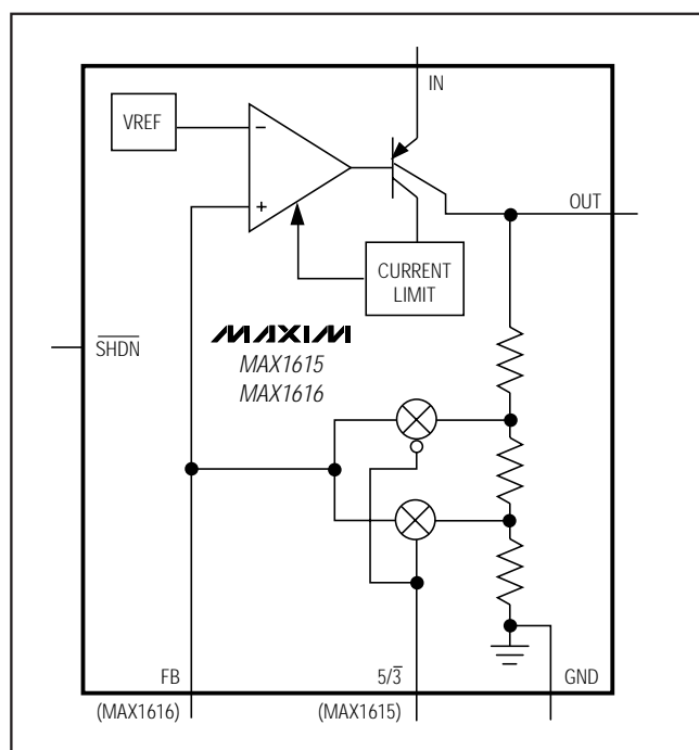
Figure 1. Functional Diagram
