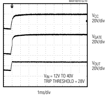
OVERVOLTAGE LIMIT ( R_{OUT} = 100\Omega , C_{IN} = 80\mu F , C_{OUT} = 10nF )
