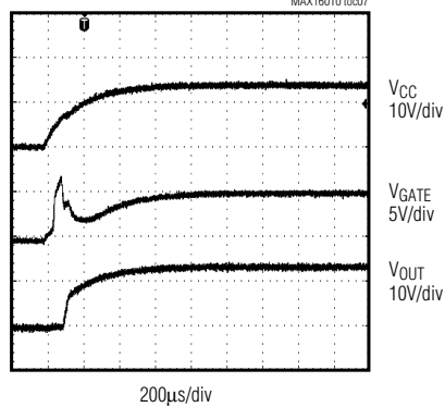
STARTUP WAVEFORM ( R_{OUT} = 100\Omega , C_{IN} = 10\mu F , C_{OUT} = 10nF )
