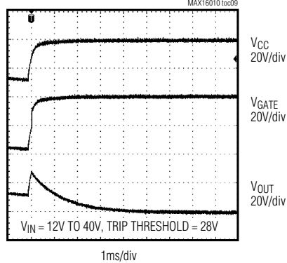
OVERVOLTAGE SWITCH FAULT ( R_{OUT} = 100\Omega , C_{IN} = 80\mu F , C_{OUT} = 10nF )
