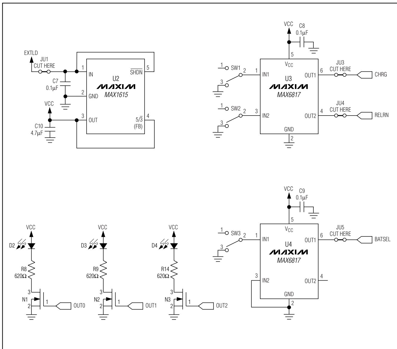
Figure 2. MAX1538 EV Kit Schematic (Sheet 2 of 2)
