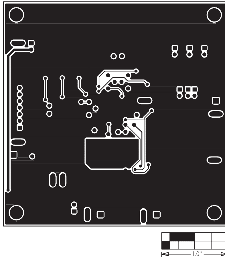
Figure 5. MAX1538 EV Kit PC Board Layout—Solder Side
