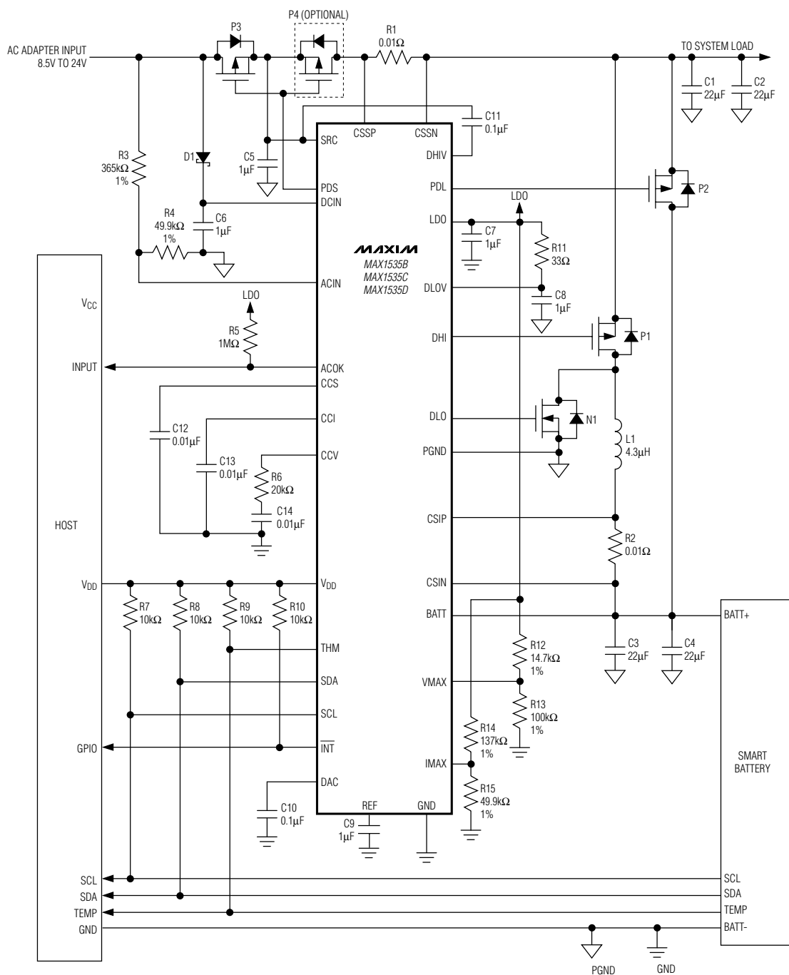
Figure 1. Standard Application Circuit
