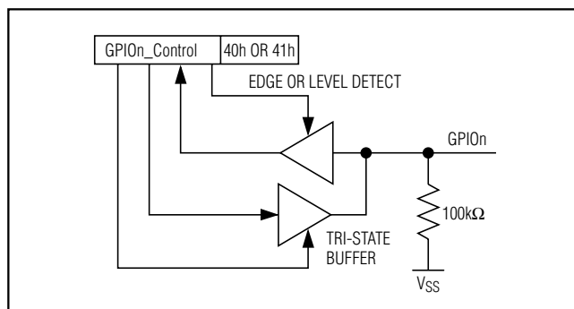
Figure 7. GPIO1 and GPIO2 Modules
