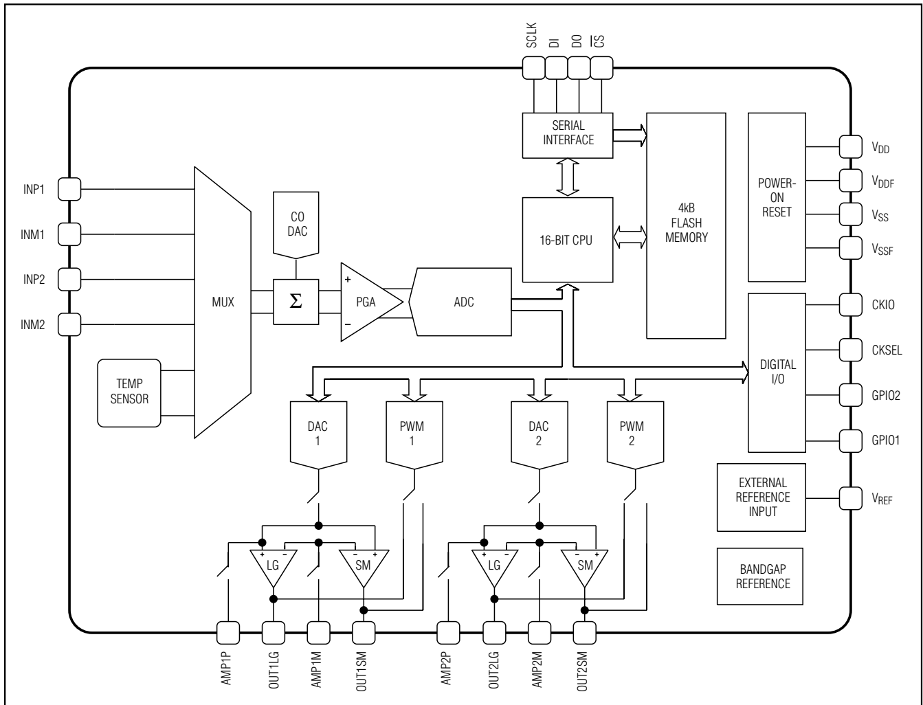
Functional Diagram
