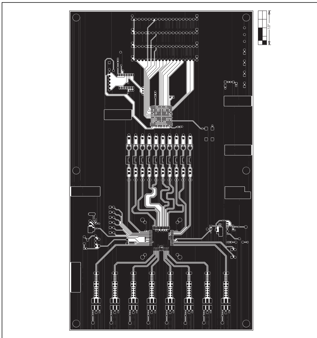
Figure 8. MAX1434/MAX1436/MAX1437/MAX1438 EV Kit PC Board Layout—Component Side
