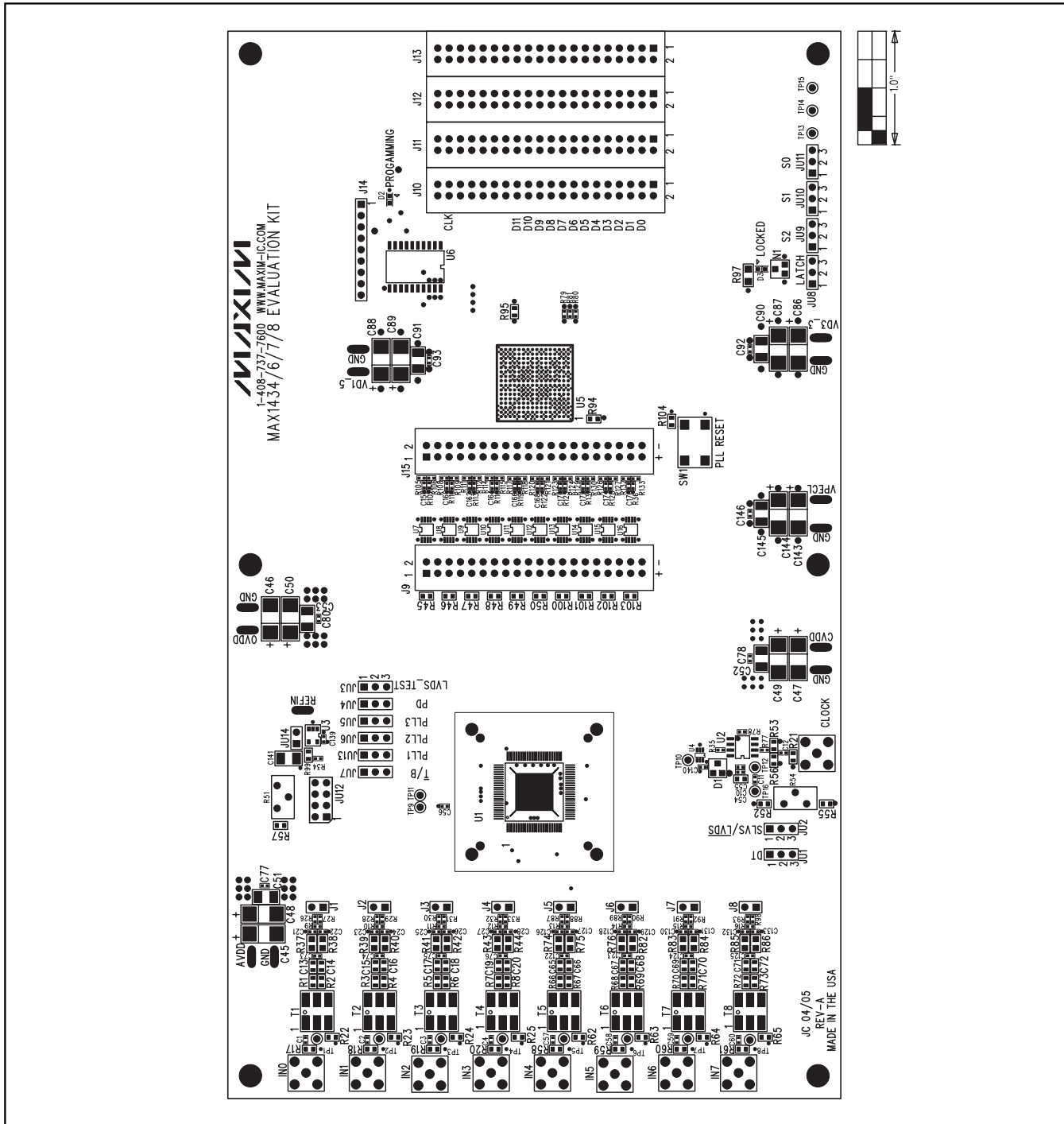
Figure 7. MAX1434/MAX1436/MAX1437/MAX1438 EV Kit Component Placement Guide—Component Side
