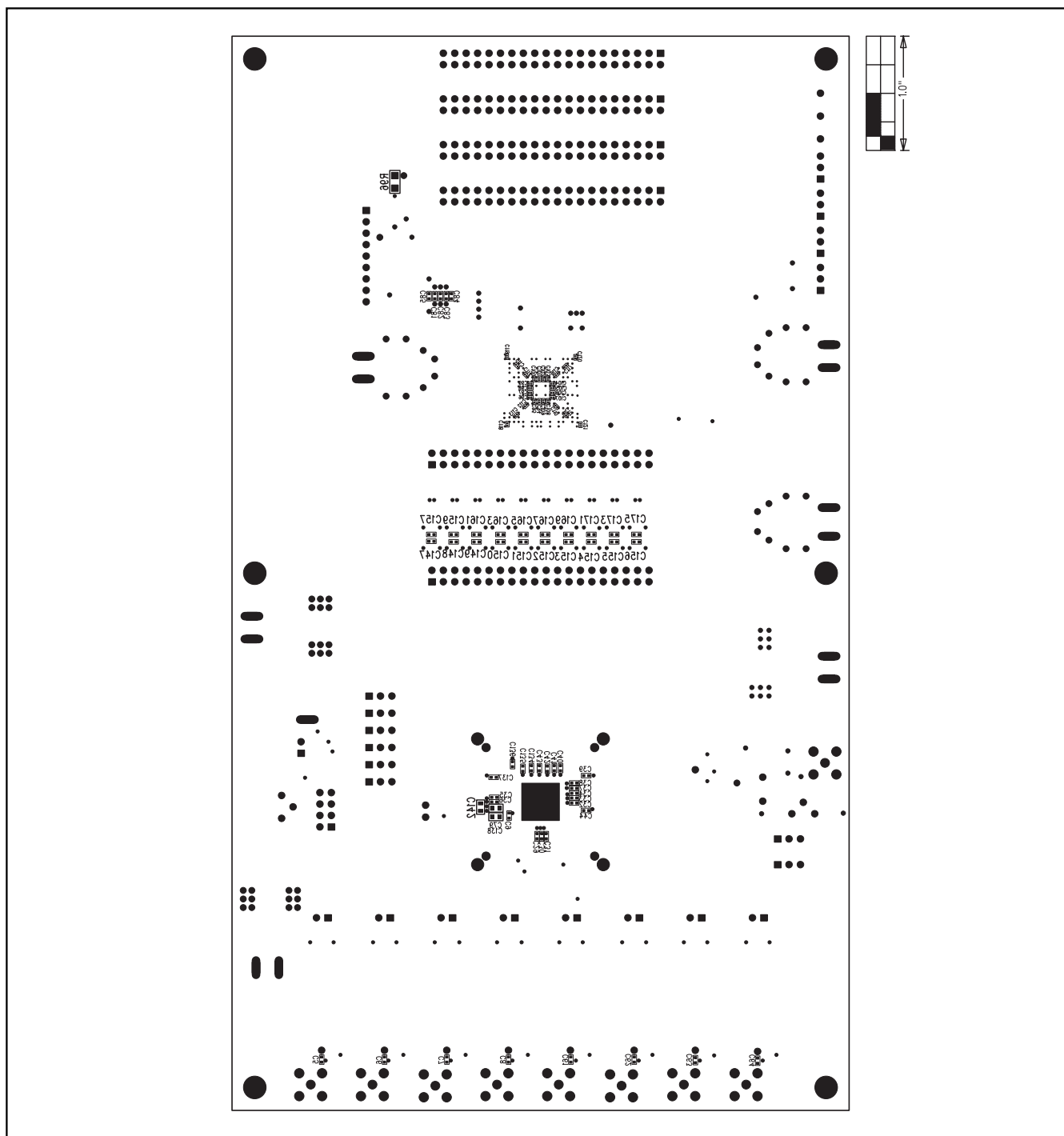
Figure 14. MAX1434/MAX1436/MAX1437/MAX1438 EV Kit Component Placement Guide—Solder Side
