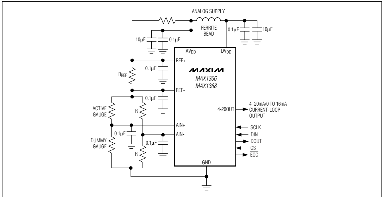
Figure 14. Strain-Gauge Application with the MAX1366/MAX1368
