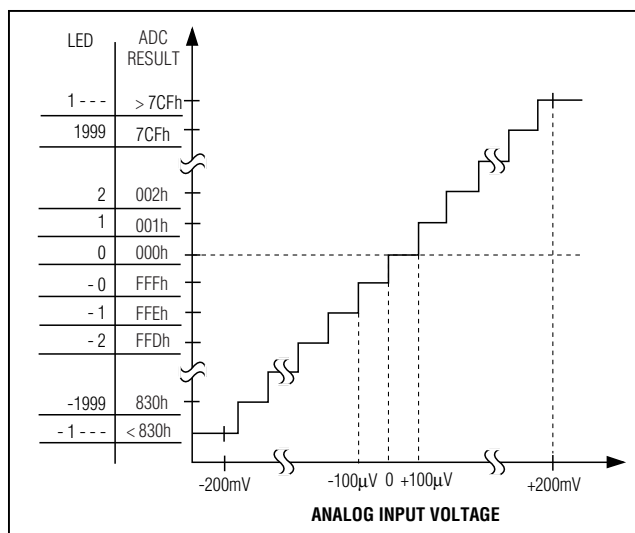
Figure 18. MAX1368 Transfer Function—±200mV Range
