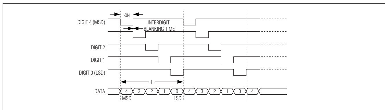
Figure 5. LED Voltage Waveform
