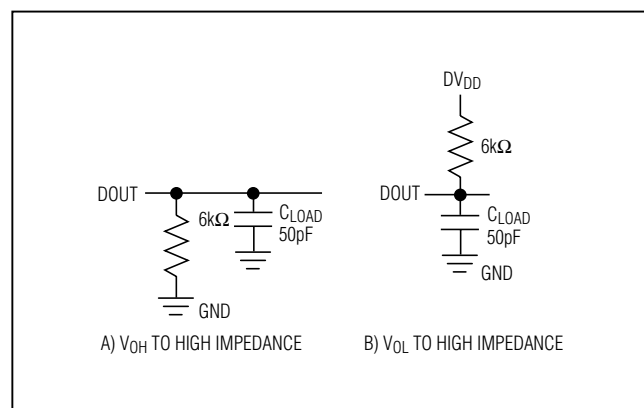
Figure 12. Load Circuits for Disable Time
