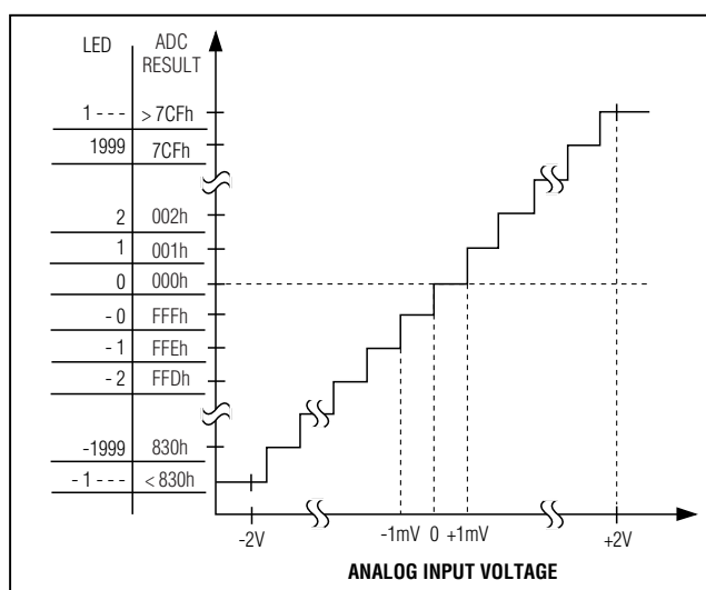
Figure 19. MAX1368 Transfer Function—±2V Range
