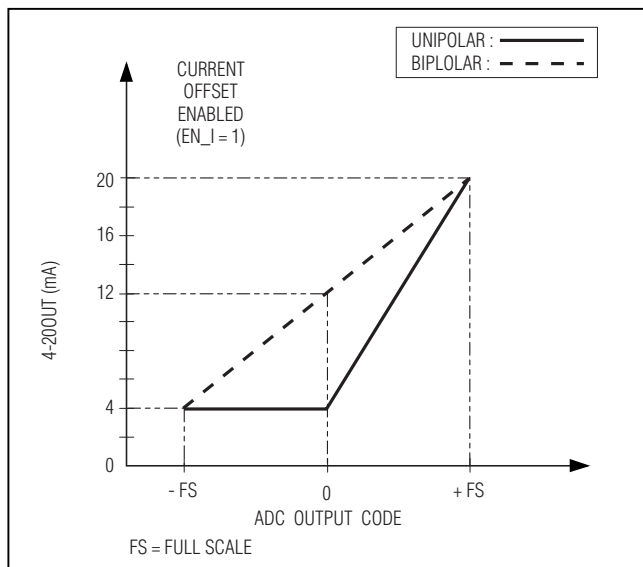
Figure 12. Output Current (4-20OUT) vs. ADC Output Code (Current Offset Enabled)
