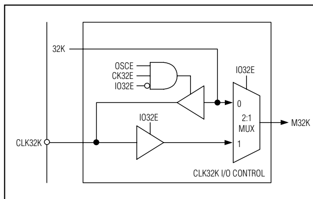
Figure 12. CLK32K I/O Block Diagram
