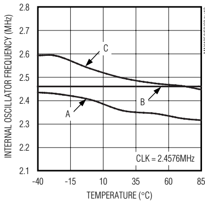
INTERNAL OSCILLATOR FREQUENCY vs. TEMPERATURE
