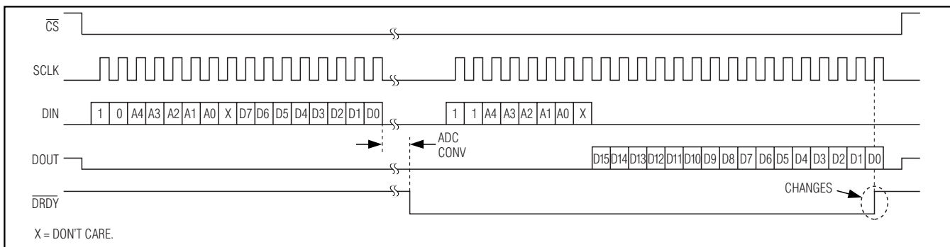
Figure 18. Performing an ADC Conversion ( \overline{\text{DRDY}} Function can be Accessed at UPIO Pins)
