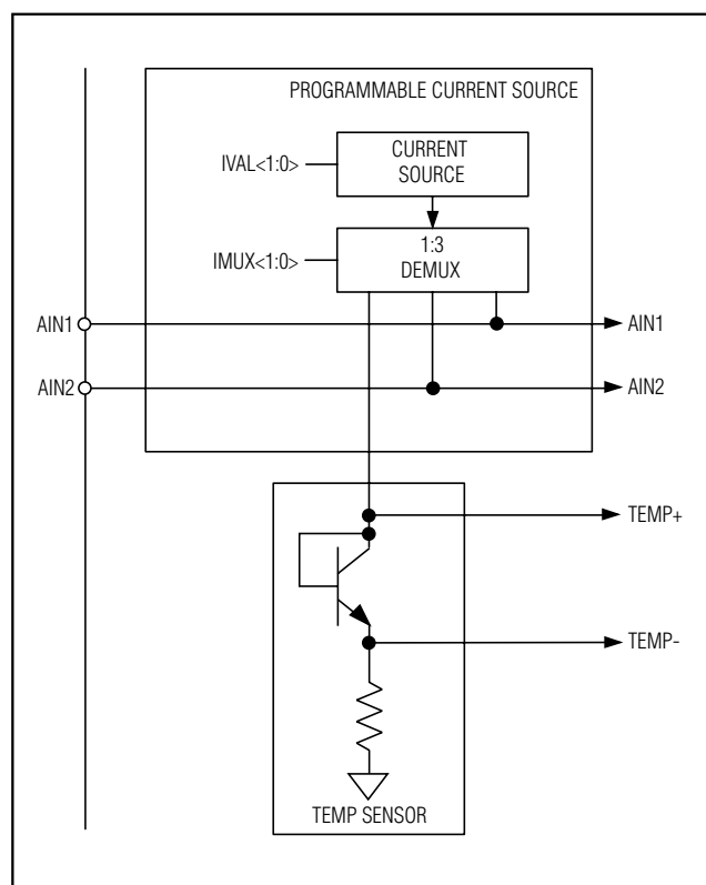
Figure 15. Temperature-Sensor Measurement Block Diagram
