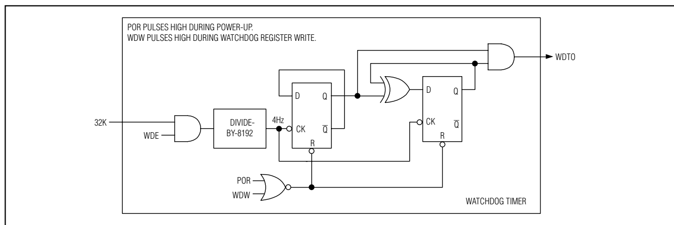
Figure 13. Watchdog Timer Block Diagram
