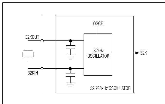
Figure 11. 32kHz Crystal-Oscillator Block Diagram
