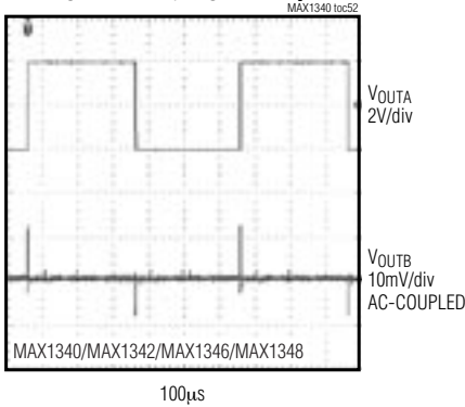
DAC-TO-DAC CROSSTALK RLOAD = 10kΩ, CLOAD = 100pF
