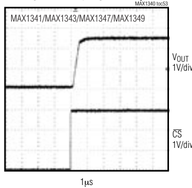
DYNAMIC RESPONSE RISE TIME RLOAD = 10kΩ, CLOAD = 100pF
