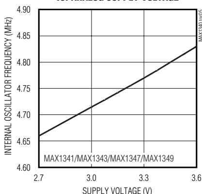
INTERNAL OSCILLATOR FREQUENCY vs. ANALOG SUPPLY VOLTAGE
