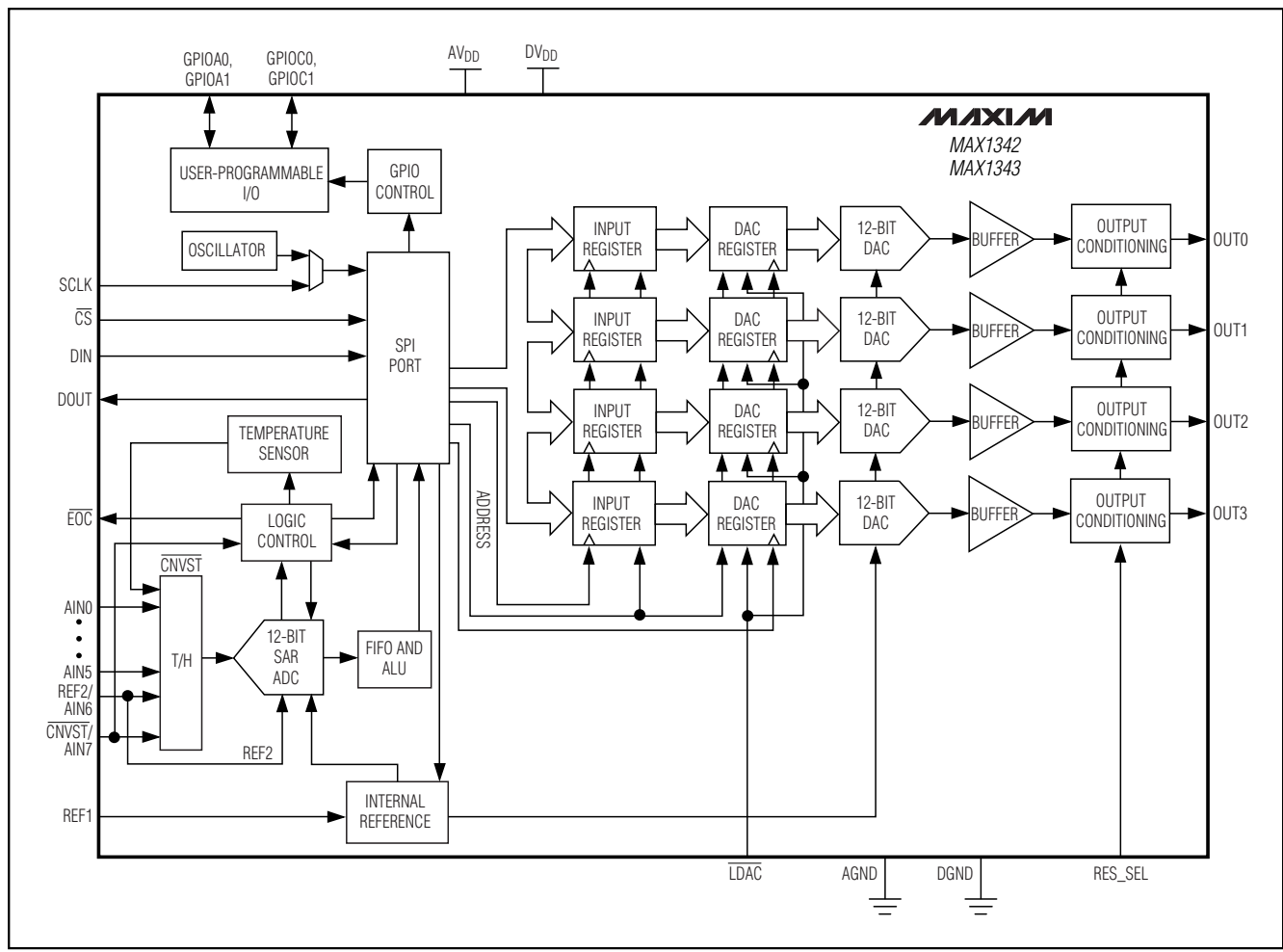
Figure 1. MAX1342/MAX1343 Functional Diagram
