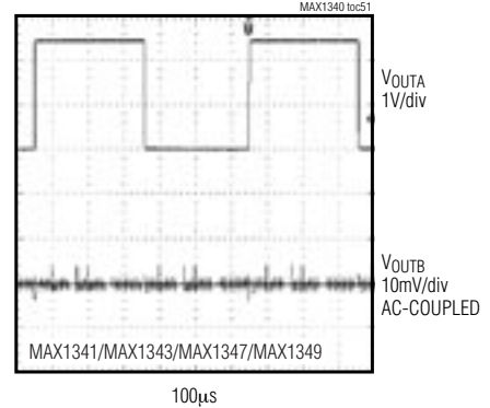
DAC-TO-DAC CROSSTALK RLOAD = 10kΩ, CLOAD = 100pF
