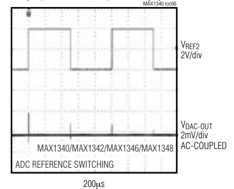
ADC REFERENCE FEEDTHROUGH ( R_{LOAD} = 10k\Omega , C_{LOAD} = 100pF )
