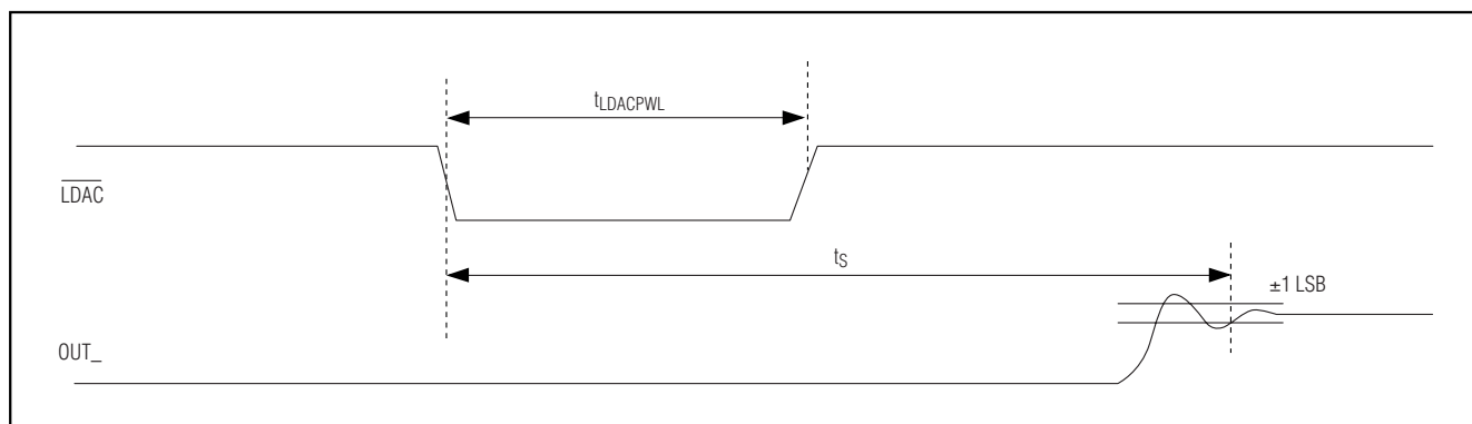
Figure 14. \overline{\text{LDAC}} Functionality
