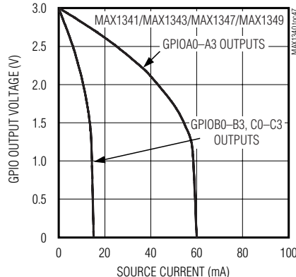
GPIO OUTPUT VOLTAGE vs. SOURCE CURRENT
