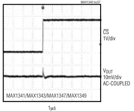
MAJOR CARRY TRANSITION RLOAD = 10kΩ, CLOAD = 100pF
