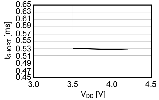
(16) t_{SHORT} - V_{DD}
