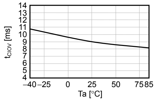
(14) t_{CI0V} - T_a
