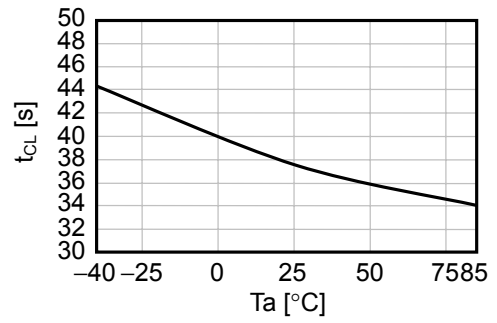
(6) t_{CL} - T_a
