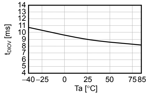
(11) t_{DIOV} - T_a
