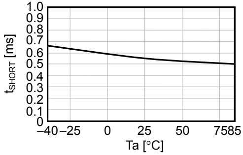
(17) t_{SHORT} - T_a
