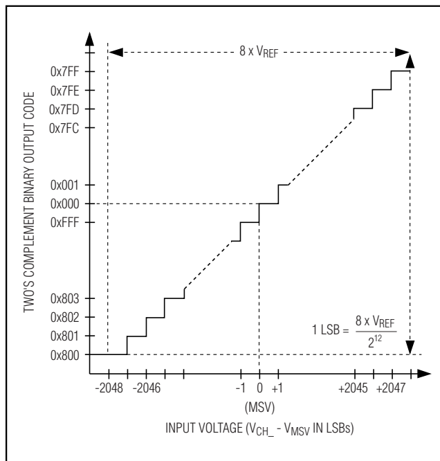
Figure 10. \pm 10\text{V} Bipolar Transfer Function
