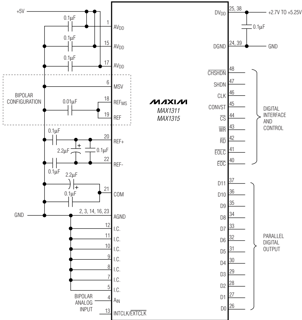
Figure 3. Typical Bipolar Operating Circuit
