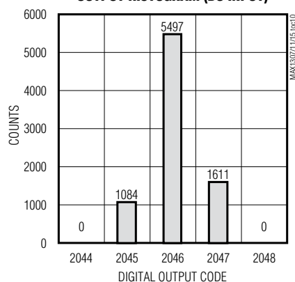
OUTPUT HISTOGRAM (DC INPUT)
