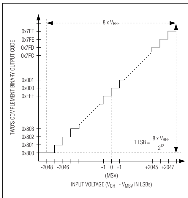
Figure 10. ±10V Bipolar Transfer Function
