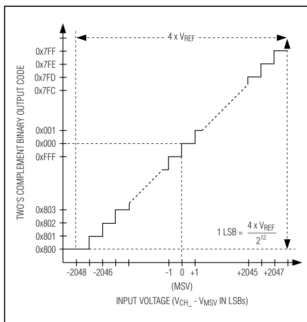
Figure 9. ±5V Bipolar Transfer Function
