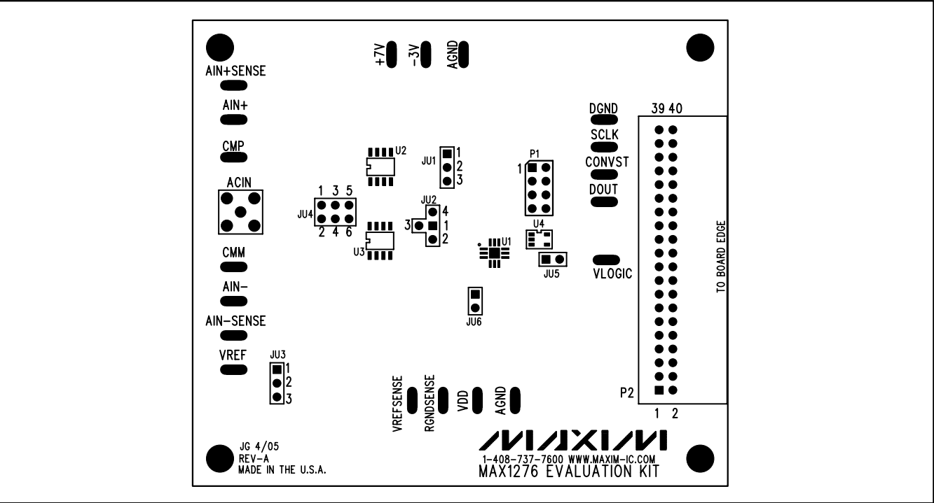
Figure 1. Jumper Locations
