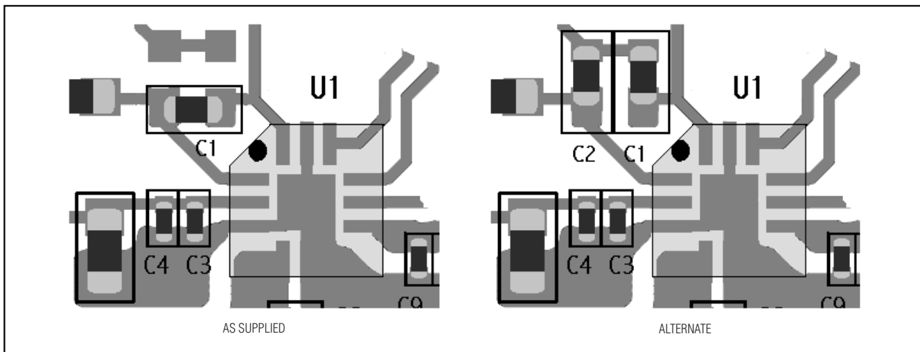
Figure 7. Input-Capacitor Options
