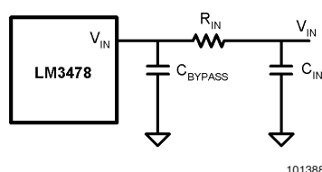
FIGURE 13. Reducing IC Input Noise
